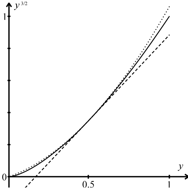
Fig. 2. The function y \rightarrow y^\alpha illustrated for \alpha = 3/2 by the full line. The lower bound given in (35) is indicated by the dashed straight line for x = 0.5 . The upper bound in (36) is indicated by the dotted line.
